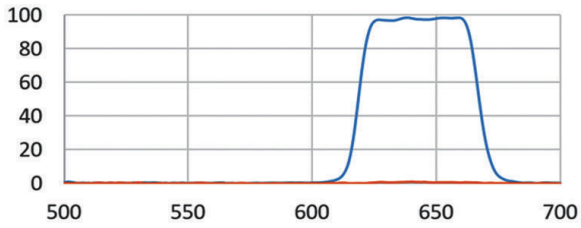
— P light — S light Red Polarized Dichroic Mirror
