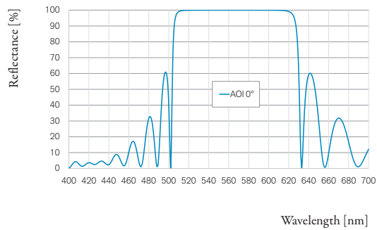
Spectral curve Mirror Nd:YAG HR532nm
